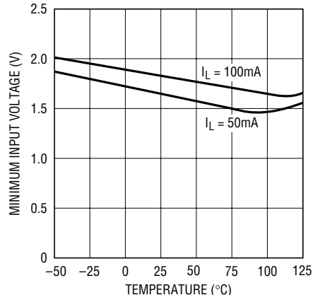
LT1761-BYP, LT1761-SD Minimum Input Voltage
