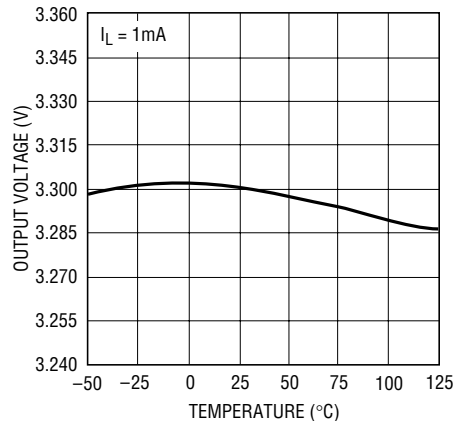
LT1761-3.3 Output Voltage
