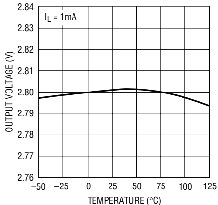
LT1761-2.8 Output Voltage
