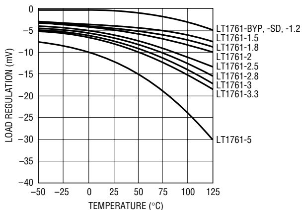
Load Regulation \Delta I_L = 1mA \text{ to } 50mA
